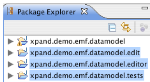
Figure 9. Generated projects
