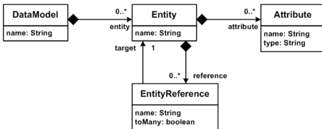
Figure 1. Sample metamodel
