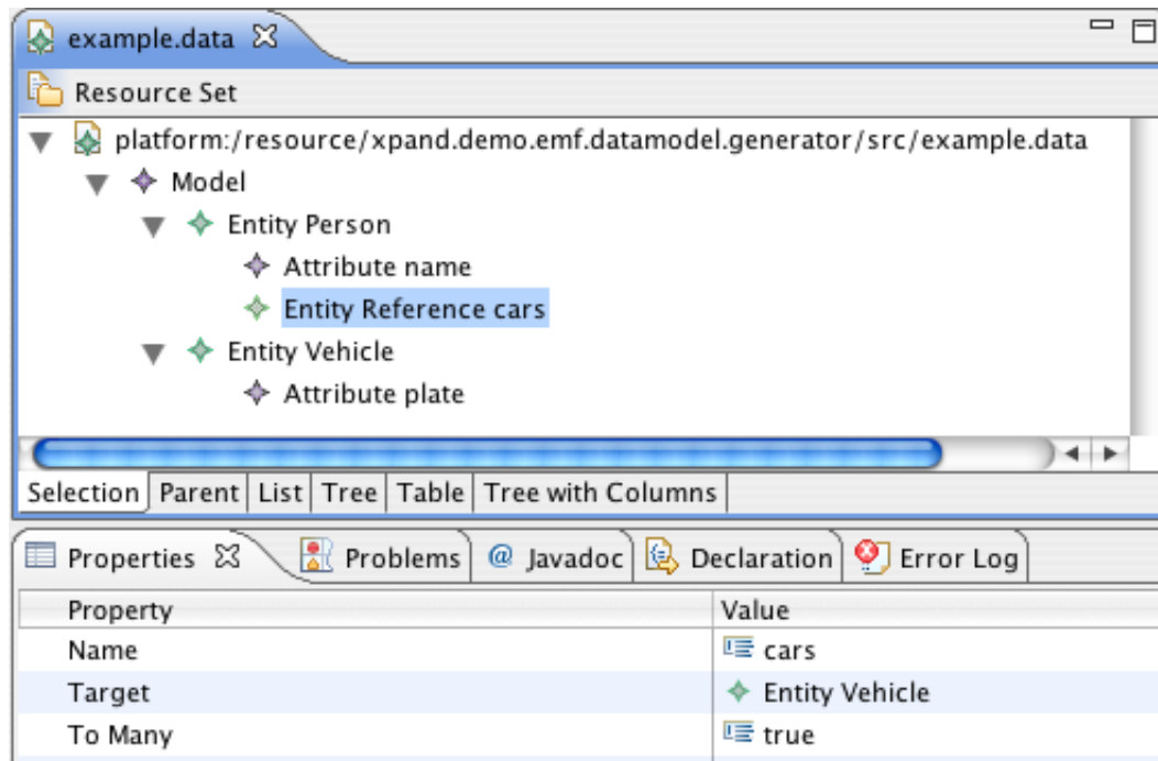
Figure 14. Sample data model
