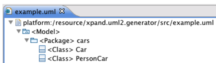
Figure 4. Example model
